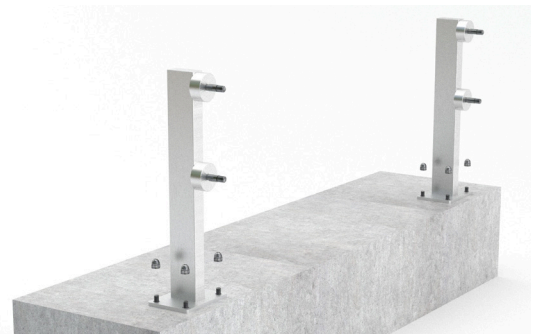
2. Mount and secure the columns.
